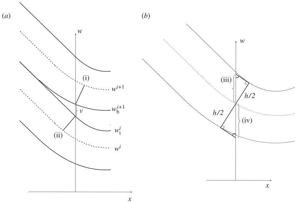
Figure 13. (a) Boundary functions determined via front propagation. (b) First-order approximation.
