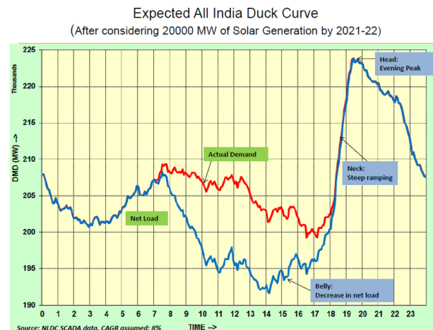
Figure 1 Expected All India Duck Curve
