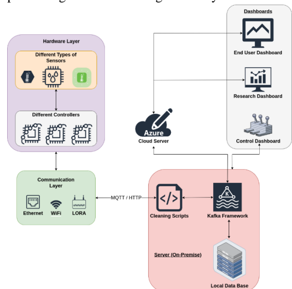
Figure 3 Control Architecture of the system
