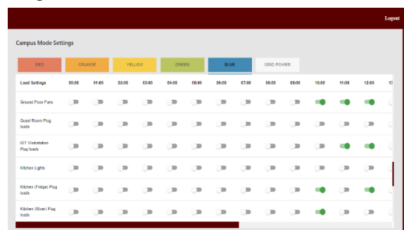
Figure 5 UI of the Campus OS to operate the scenarios
