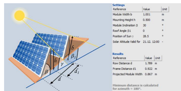
Figure 7: Photovoltaic panels parameters
