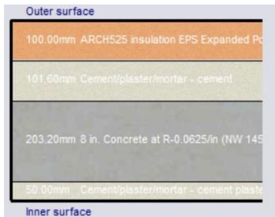
Figure 5: Detail of external wall after applying insulation
