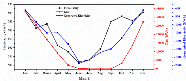
Figure 9: Fuel usage breakdown of retrofitted RB by PV panel; Electricity (black curve), gas (red curve), and generated power (blue curve)
